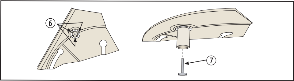
Figure 3.4: Ceiling Tamper
