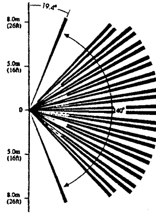
EWA-1 STANDARD LENS (OPTIONAL)
