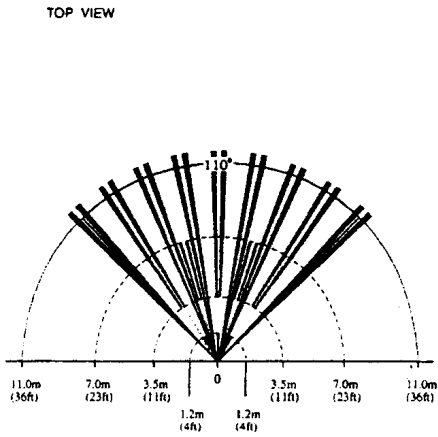
WA-1 STANDARD LENS
